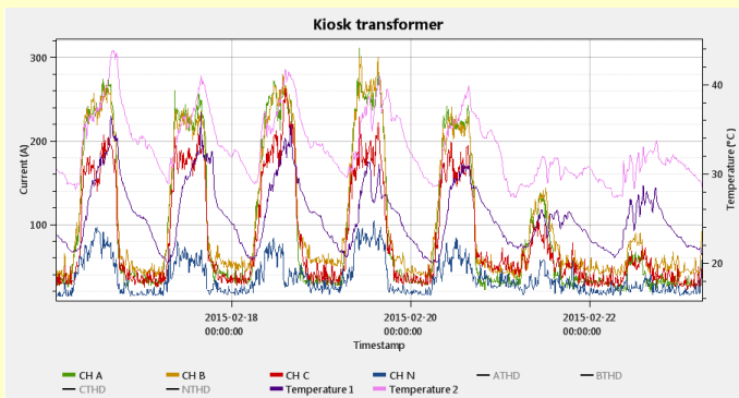
Figure 3: Reporting - kiosk transformer weekly profile
